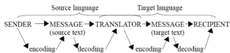
Figure 1: Translation Procedure
