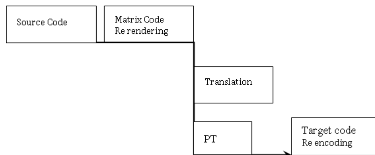
Figure 2: Translation Matrix
